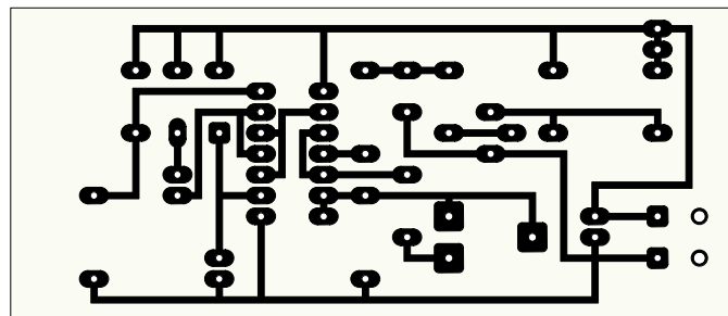
track pattern: looking through the pcb as if it was transparent
